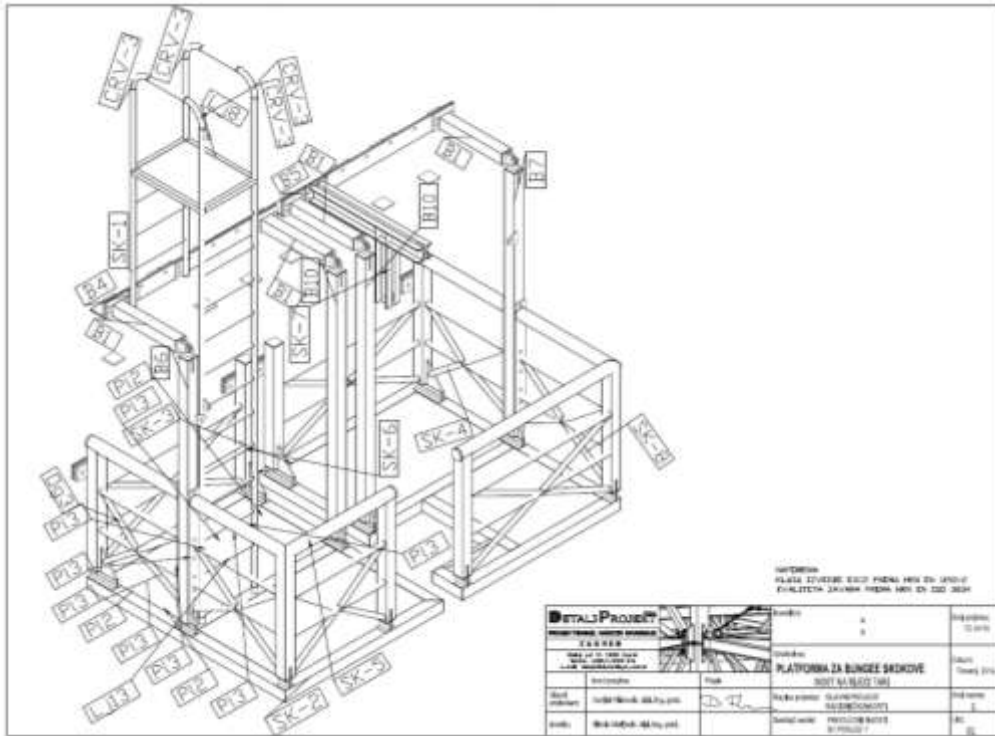
Slika 4 technical drawing of full assembly
