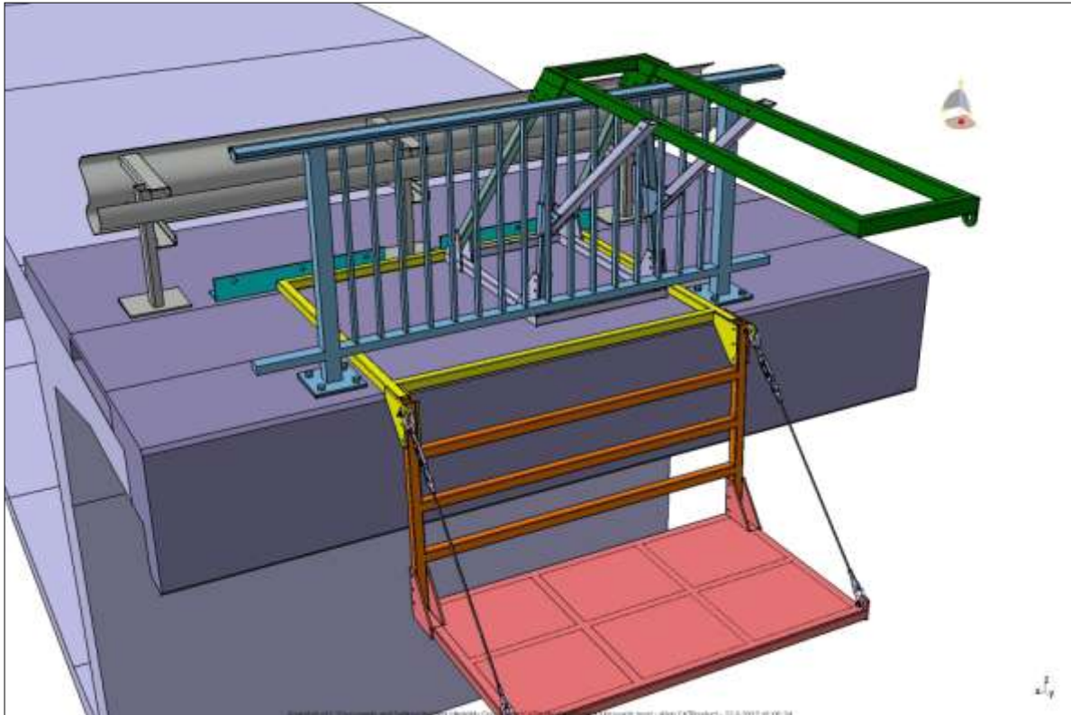
Slika 1 3D model of the platform in Dubrovnik
