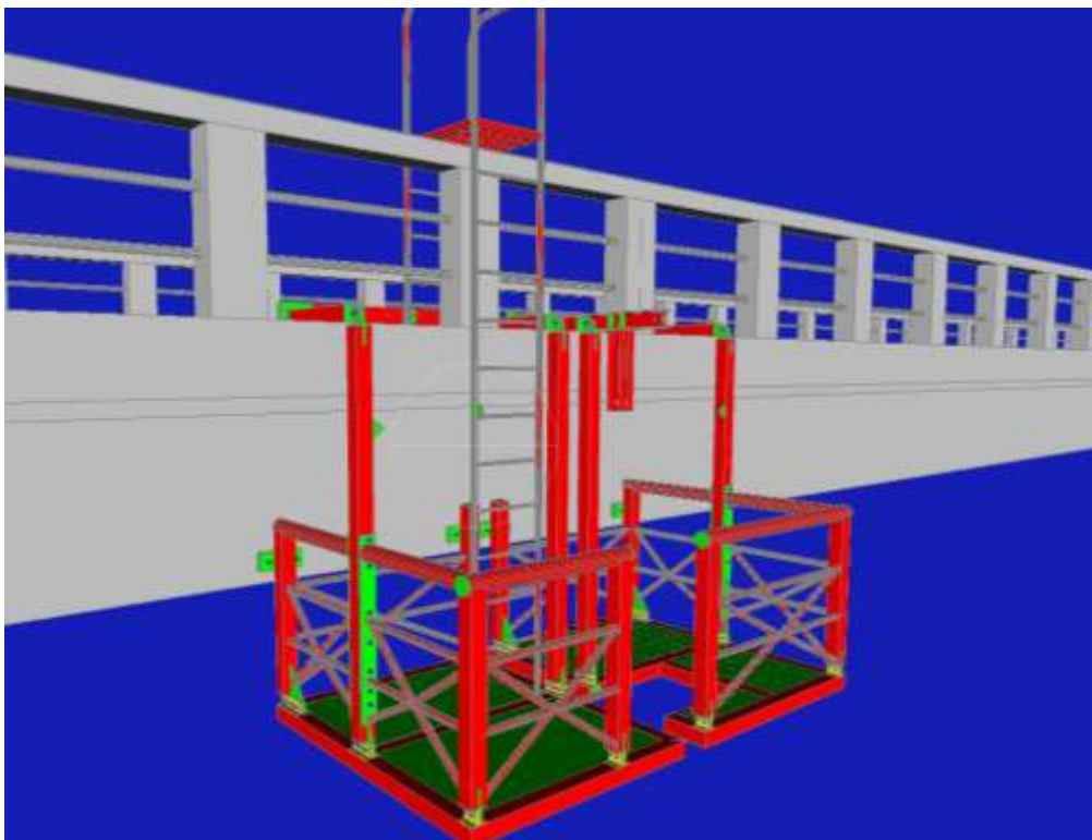
Slika 5 3D model of the platform
